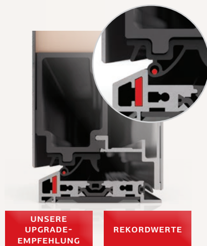
MAGNET WEATHERSEAL
